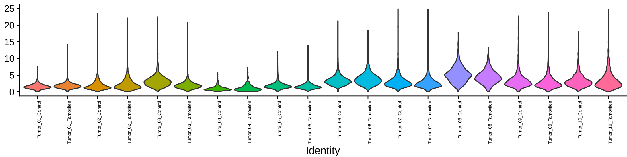
percent.mt
