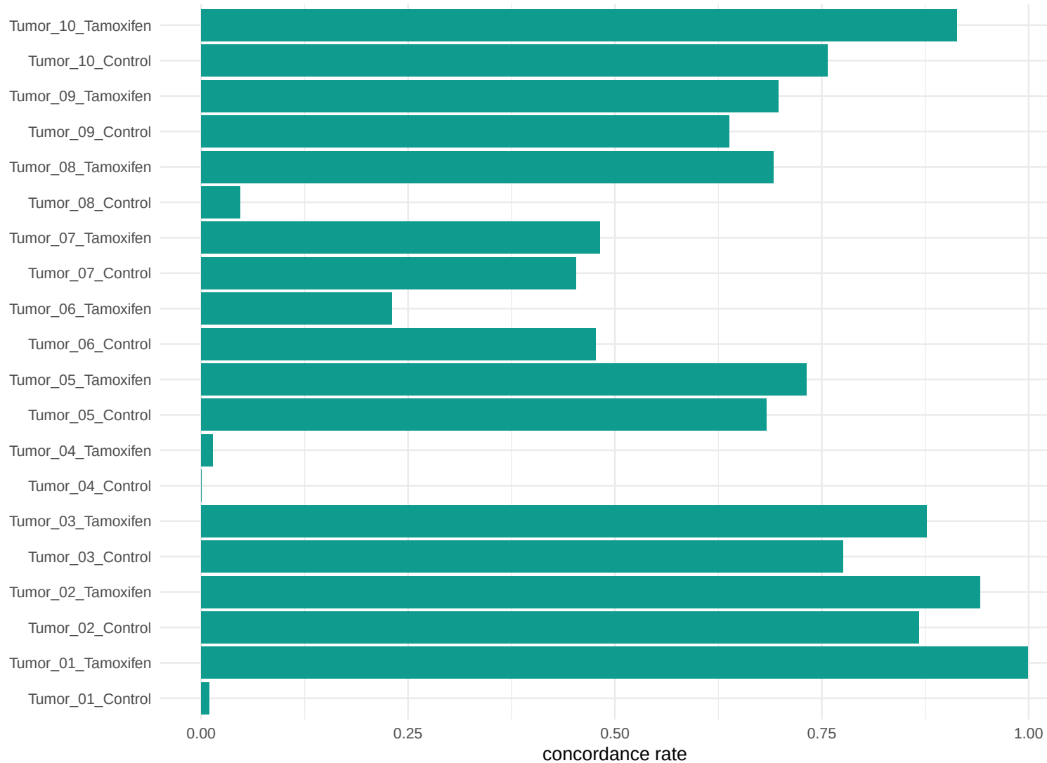
Primary (InferCNV) vs. sensitivity (CopyKAT) malignancy concordance
