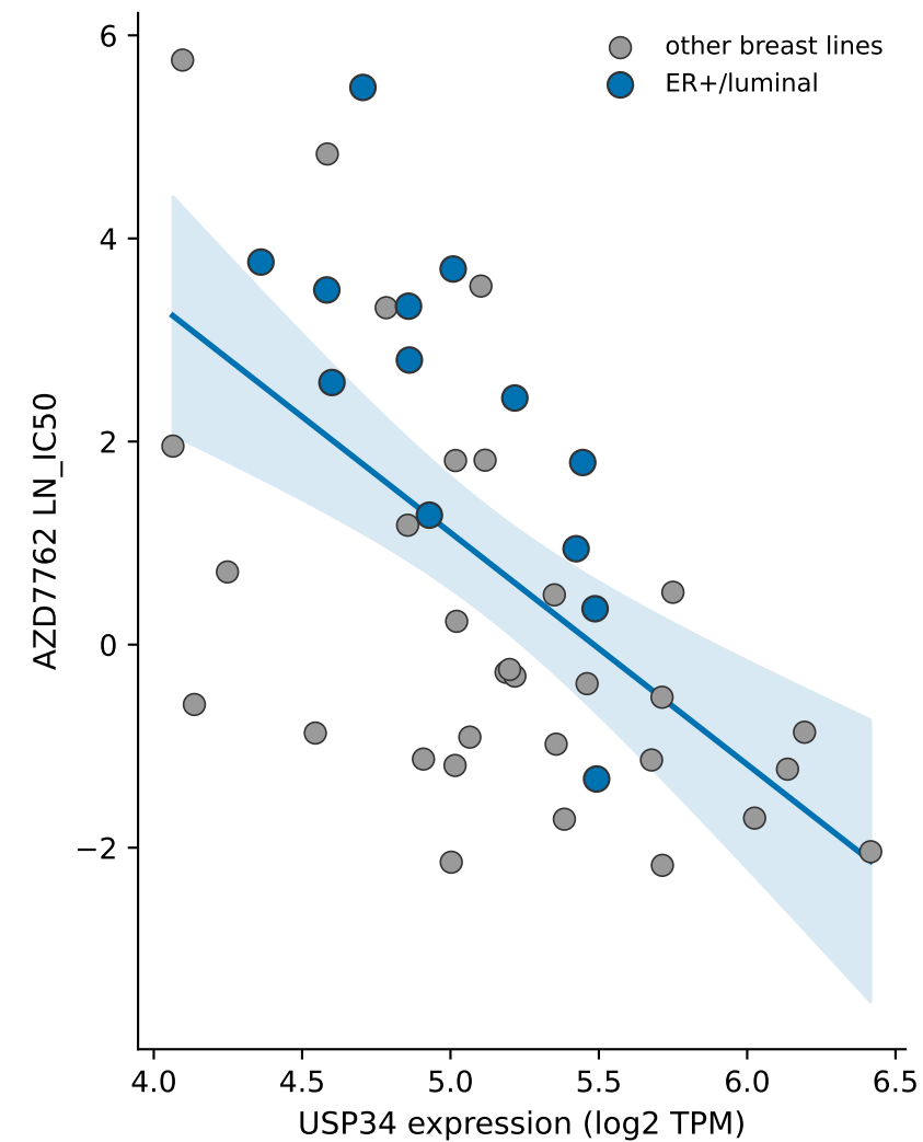
B. USP34 x AZD7762 ( \rho=-0.59 , FDR=0.008, n=44)
