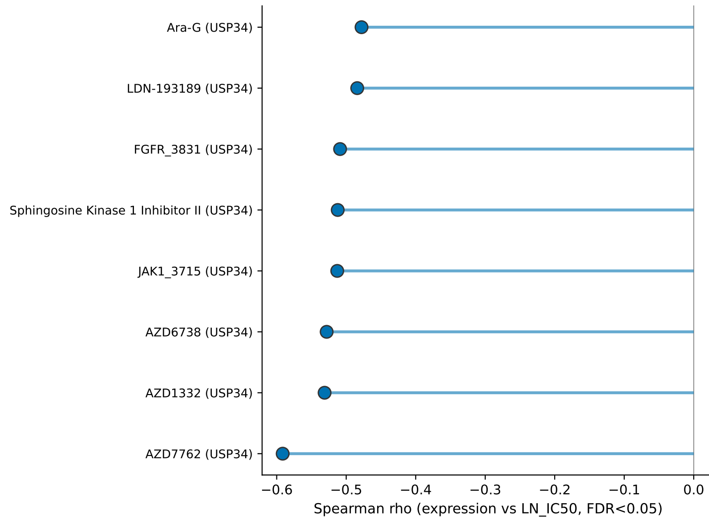
A. Top FDR-significant GDSC drug associations
