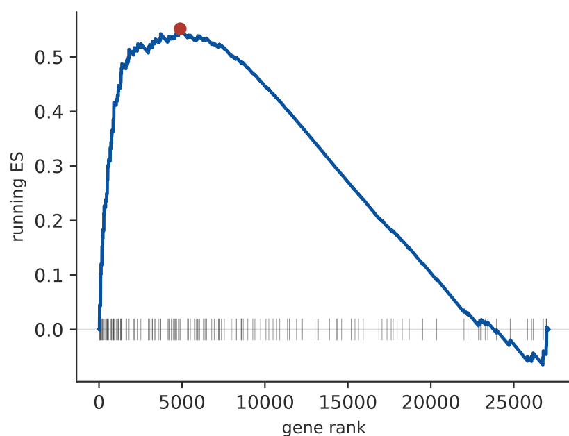
GSE111151: EMT
