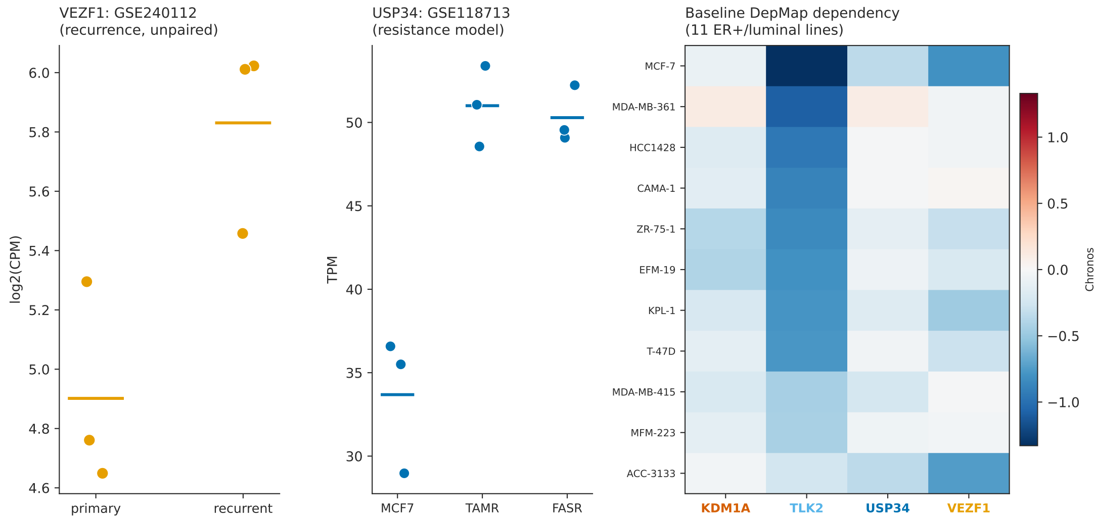
Panels A-B: real human/cell-line evidence supporting VEZF1 and USP34 respectively. Panel C: baseline dependency for all 4 focus genes side by side -- a different, orthogonal quantity, not more of the same evidence.
