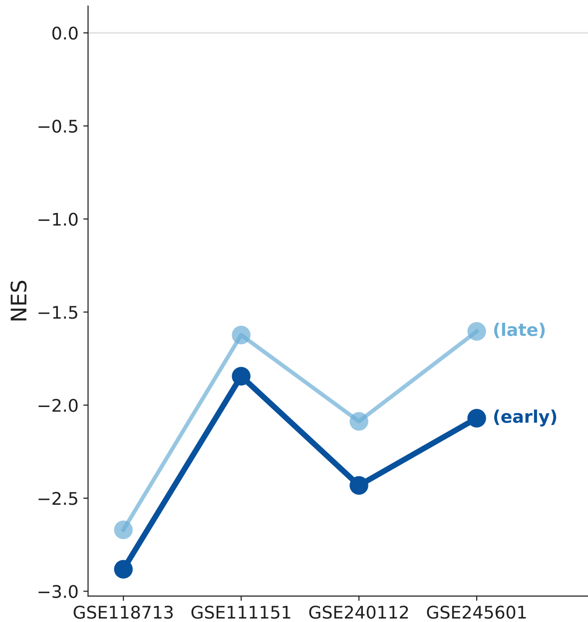
Estrogen response falls in every context
