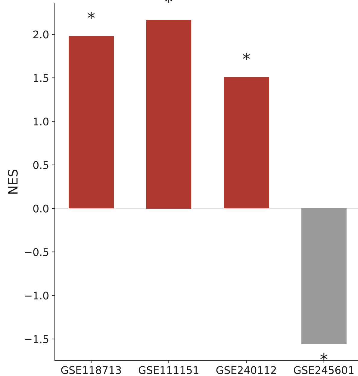
EMT rises in resistance and recurrence, falls acutely
