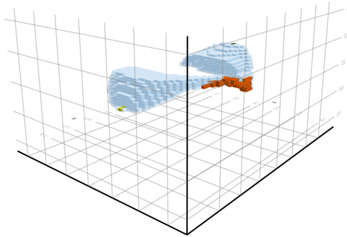
Figure 6.11: Allen-Cahn Morse interval, View 2
