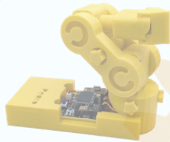
Lesson #2 Pedro Board
