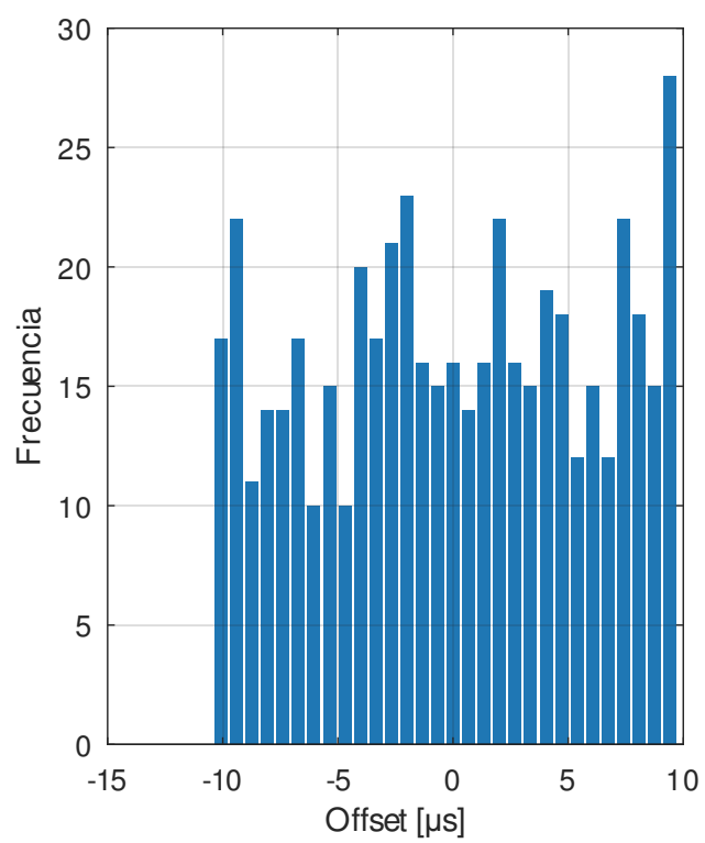
Exel (baseline)
