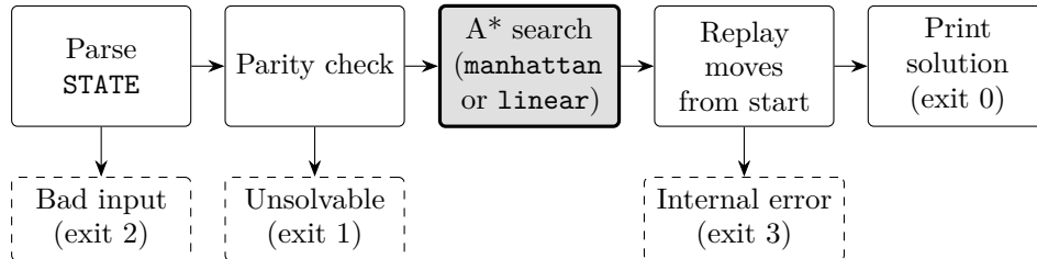
Figure 2: How solve handles one input. A* (shaded) is the only step that searches.
