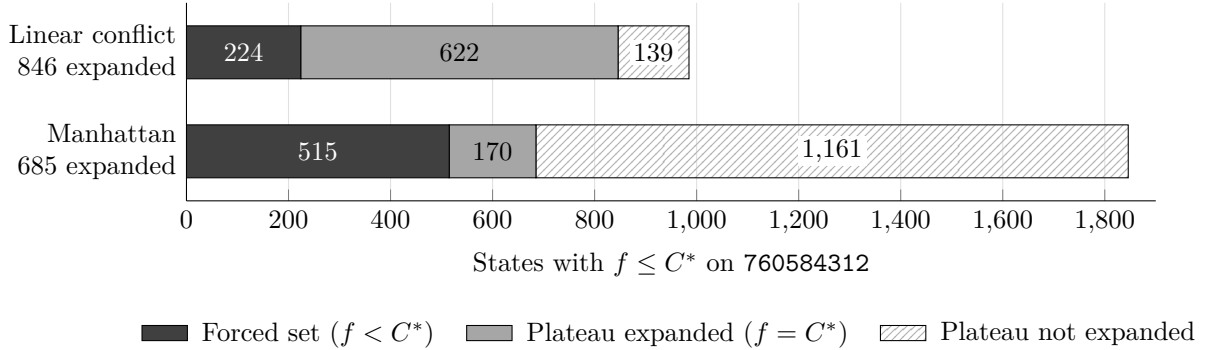
Figure 3: Where the expansions go on 760584312. Linear conflict has the smaller forced set and the smaller plateau, but A* expands most of its plateau before popping the goal.
