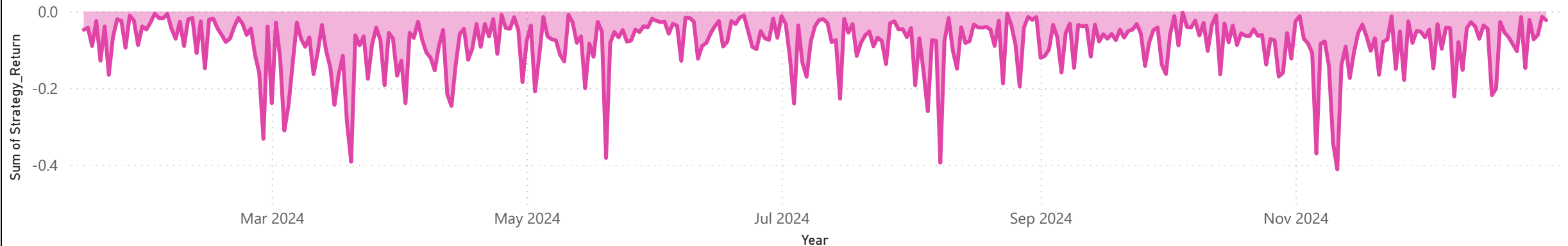
Risk View
