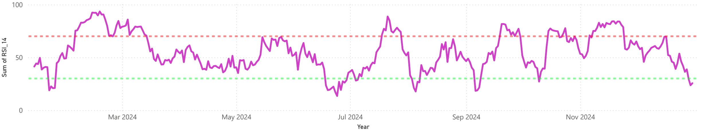
RSI Indicators
