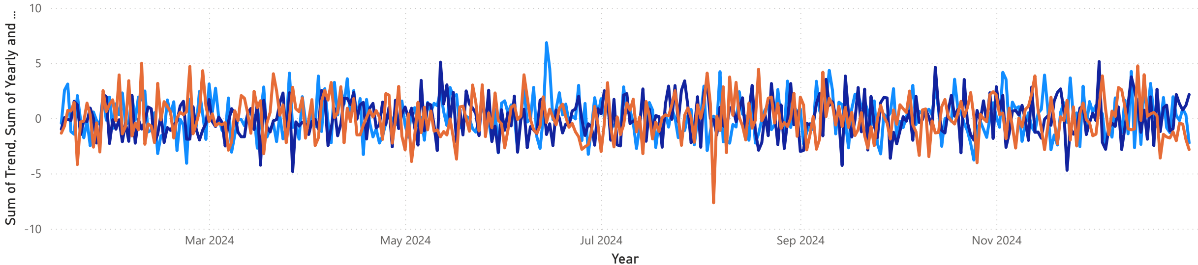
Prophet Explainability
