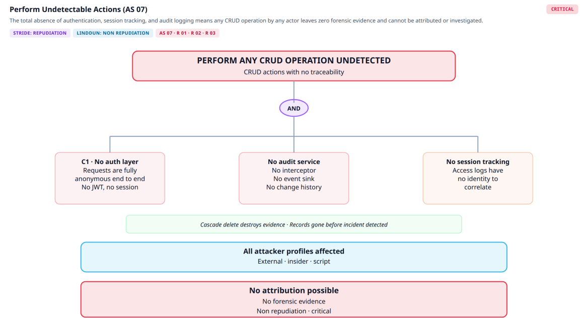
Figure 1.11: Attack tree 6 – Perform Undetectable Actions
