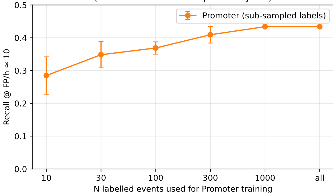
FRDR Promoter — label-efficiency curve (5 seeds × 5-fold GroupKFold by file)
