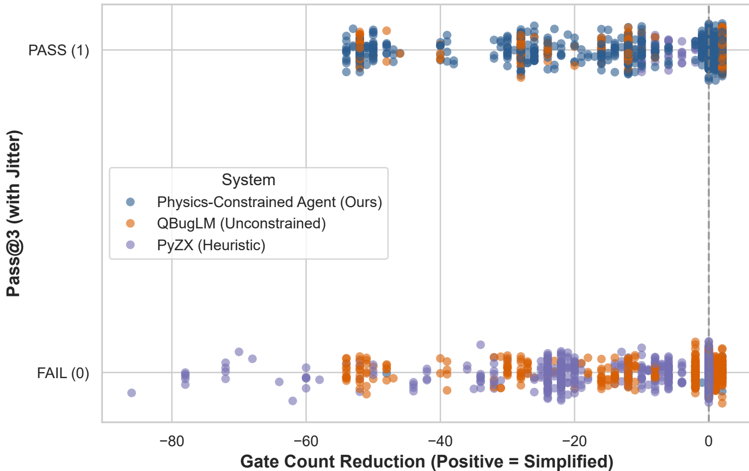
Gate Count Reduction vs. Repair Success (Pass@3)
