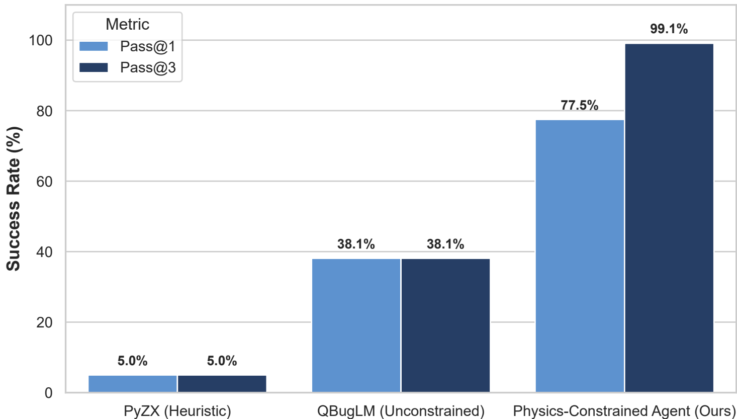
Repair Success Rates (Pass@1 vs. Pass@3)
