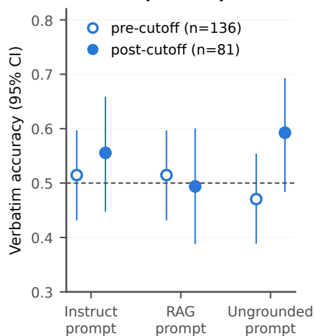
(b) LLM: pre- vs. post-cutoff CVEs
