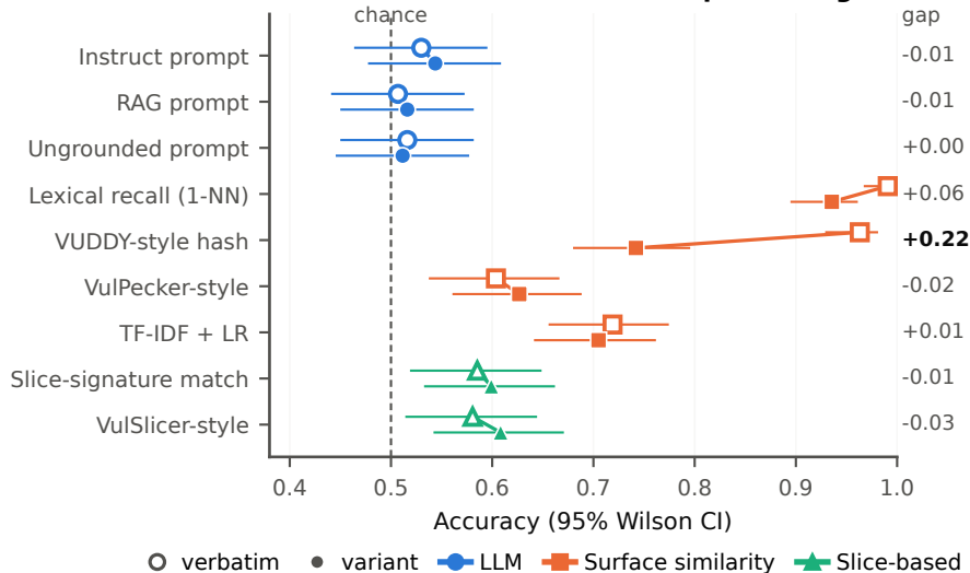
(a) Verbatim vs. certified slice-preserving variant
