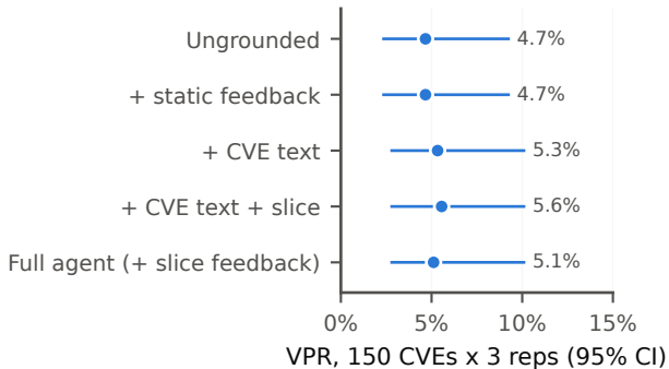
(b) Validated-patch rate
