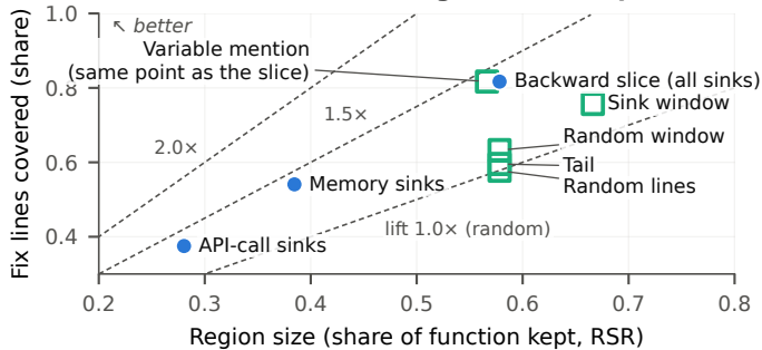
(a) Which sinks, which region? All 760 pairs
