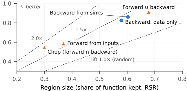
(b) Which direction? 338 pairs with a forward slice
