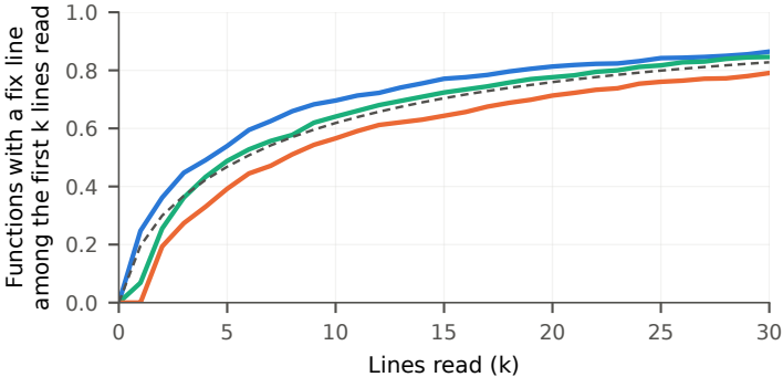
(a) BigVul, all 760 deletion pairs
