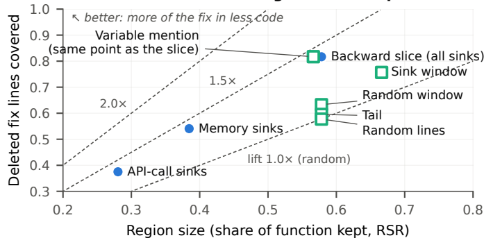
(a) Which sinks, which region? All 760 pairs
