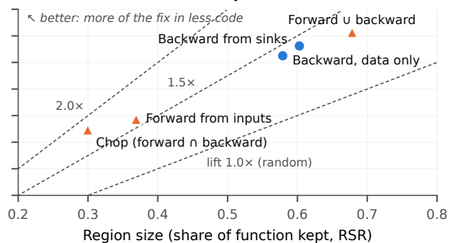
(b) Which direction? 338 pairs with a forward slice
