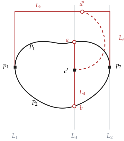
Figure 5: The configuration behind “a Jordan curve separates”. Squares mark p_1, p_2, c' ; circles mark a, b, d' . Every square is joined to every circle by one of nine internally disjoint arcs — four subarcs of C , two halves of L_4 , two pieces of L_5 , and L_6 — so the picture is a plane subdivision of K_{3,3} , which cannot exist. The dashed L_6 is the hypothesis being refuted — it is assumed to reach L_5 from L_4 without meeting C — so no drawing of it can be faithful; here it is shown crossing C on the right.
