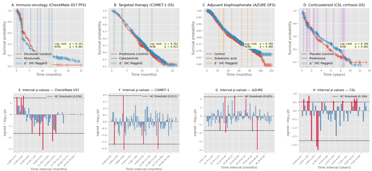
Fig. 1. Higher Criticism detects non-proportional hazard departures across four clinical datasets with distinct temporal patterns. Top row (A–D): Kaplan-Meier curves with HCHG-flagged intervals (shaded). Bottom row (E–H): per-interval \text{signed } -\log_{10}(\text{hypergeometric } p\text{-value}) . Upward bars mark excess events in the treatment arm, downward bars mark excess in the control arm. Dashed lines are the per-direction HCHG thresholds; bars reaching beyond either line are highlighted in red and coincide exactly with the intervals shaded above. (A,E) CheckMate 057 PFS (nivolumab vs. docetaxel, n = 582 ); log-rank p = 0.351 , HCHG p = 0.001 . Curves cross at \sim 3 months before nivolumab gains a durable late advantage. (B,F) COMET-1 OS (cabozantinib vs. prednisone, n = 1028 ); log-rank p = 0.262 , HCHG p = 0.014 . Early OS advantage (months 3–7) during bone-lesion response, fading as resistance develops. (C,G) AZURE DFS (zoledronic acid vs. control, n = 3359 ); log-rank p = 0.305 , HCHG p = 0.005 . Menopause-dependent benefit accumulates in months 20–60. (D,H) CSL OS (prednisone vs. placebo, liver cirrhosis, n = 446 ); log-rank p = 0.384 , HCHG p = 0.002 . Time-varying corticosteroid effect with multiple curve crossings; fully public raw individual patient data (CRAN timereg / SurvSet ). In every dataset the log-rank test is non-significant while HCHG is significant. For the first three, individual patient data were reconstructed via Guyot et al. [2012].
