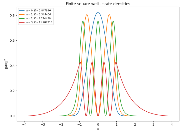
Figure 20: Probability densities |\psi(x)|^2 for the first four finite square well states. The densities show both interior oscillation and exterior exponential leakage.
