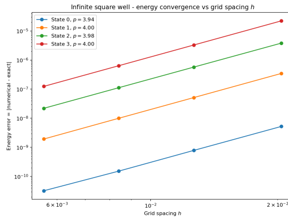
Figure 4: Energy error versus grid spacing h for the infinite square well.
