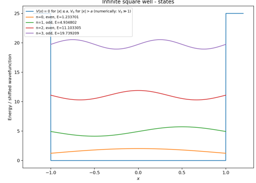
Figure 2: Wavefunctions for the first four infinite-square-well states.
