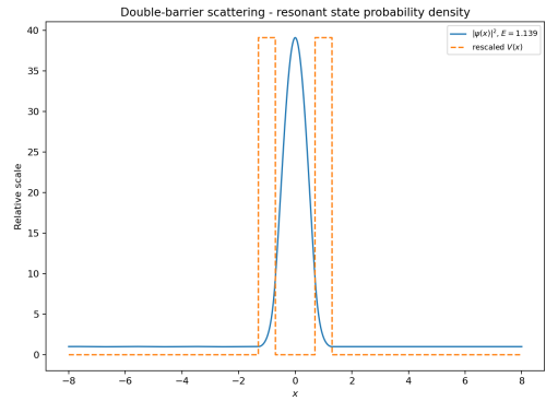
Figure 13: Probability density at the first resonant energy.
