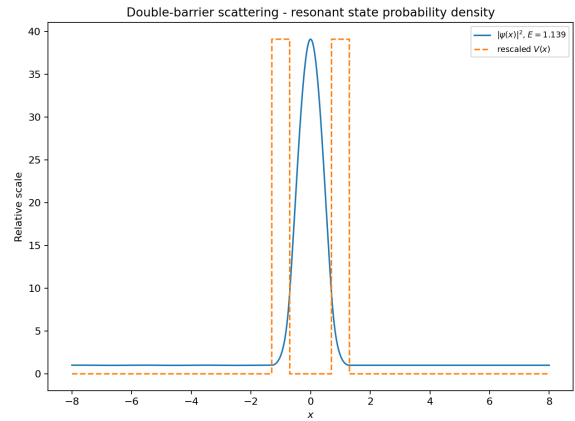
Figure 13: Probability density at the first resonant energy.
