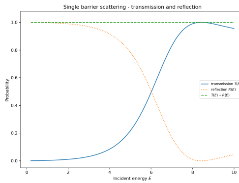
Figure 11: Transmission and reflection probabilities for a finite rectangular barrier.
