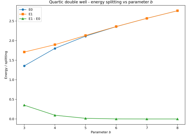
Figure 9: Lowest two double-well energies and their splitting versus b .
