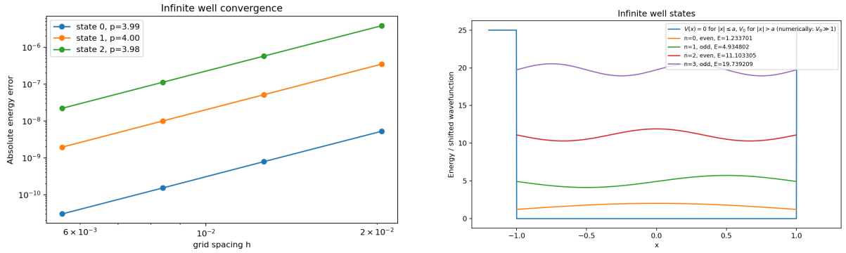
Figure 4: Convergence of the energy error as a function of grid spacing h . The slopes are close to fourth order, as expected for the Numerov method.
