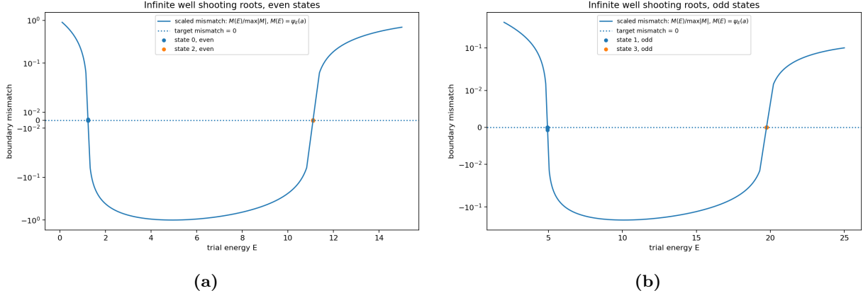
Figure 3: Boundary mismatch functions for even (a) and odd (b) states. The zero crossings correspond to the physical eigenvalues found by the shooting method.
