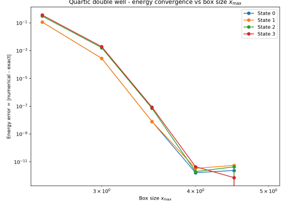
Figure 20: Dependence of the double-well energy errors on box size, measured relative to a larger-box reference calculation at approximately fixed grid spacing. The errors decrease rapidly as the domain is enlarged and then reach a numerical plateau.
