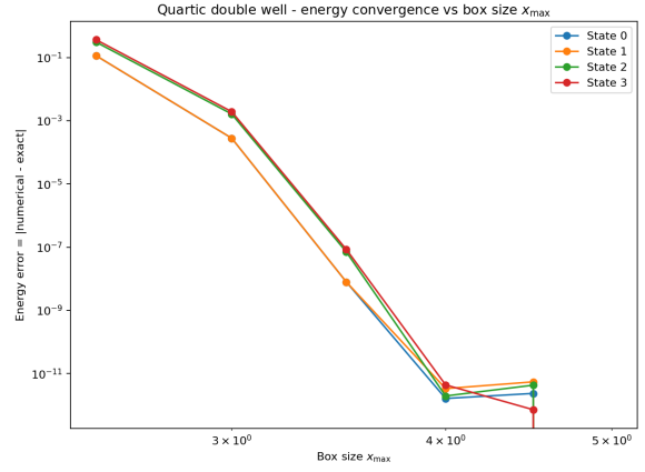
Figure 20: Dependence of the double-well energy errors on box size. The errors decrease rapidly as the domain is enlarged and then reach a numerical plateau.
