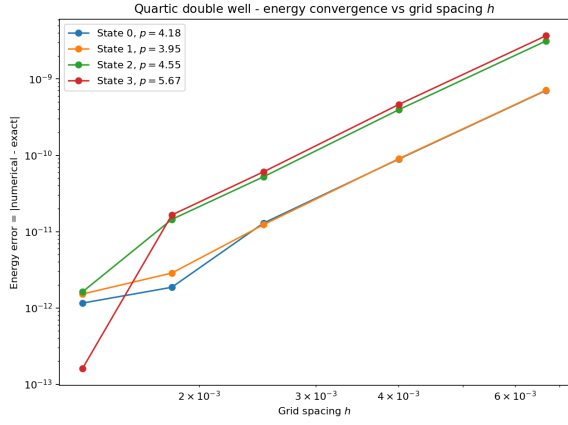
Figure 19: Grid convergence for the quartic double well. The energy errors decrease with high-order behavior under successive grid refinement.
