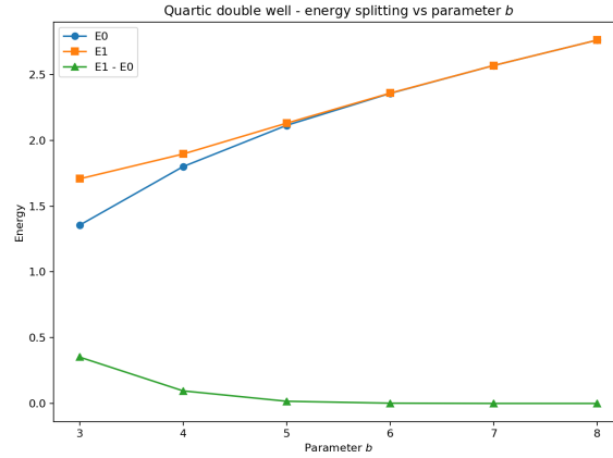
Figure 21: Energy splitting between the two lowest double-well states as the parameter b is varied. The splitting decreases as the barrier becomes stronger, consistent with tunneling suppression.
