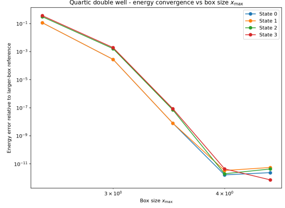
Figure 20: Dependence of the double-well energy errors on box size, measured relative to a larger-box reference calculation at approximately fixed grid spacing. The reference point itself has identically zero error and is therefore omitted from the log-scale plot. The errors decrease rapidly as the domain is enlarged and then reach a numerical plateau.
