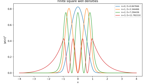
Figure 20: Probability densities |\psi(x)|^2 for the first four finite square well states. The densities show both interior oscillation and exterior exponential leakage.
