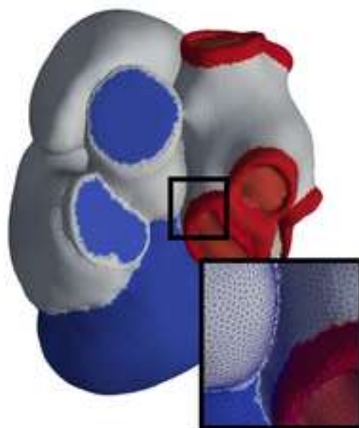
(b) Full volumetric mesh
