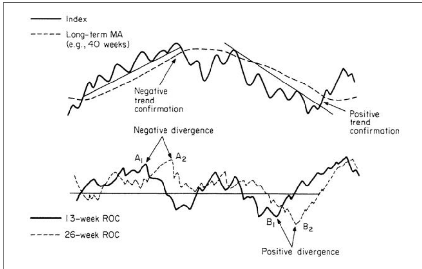
FIGURE 13.15 Complex Divergence
