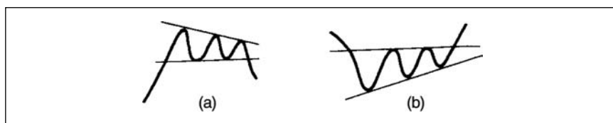
FIGURE 8.39 Right-Angled Triangles
