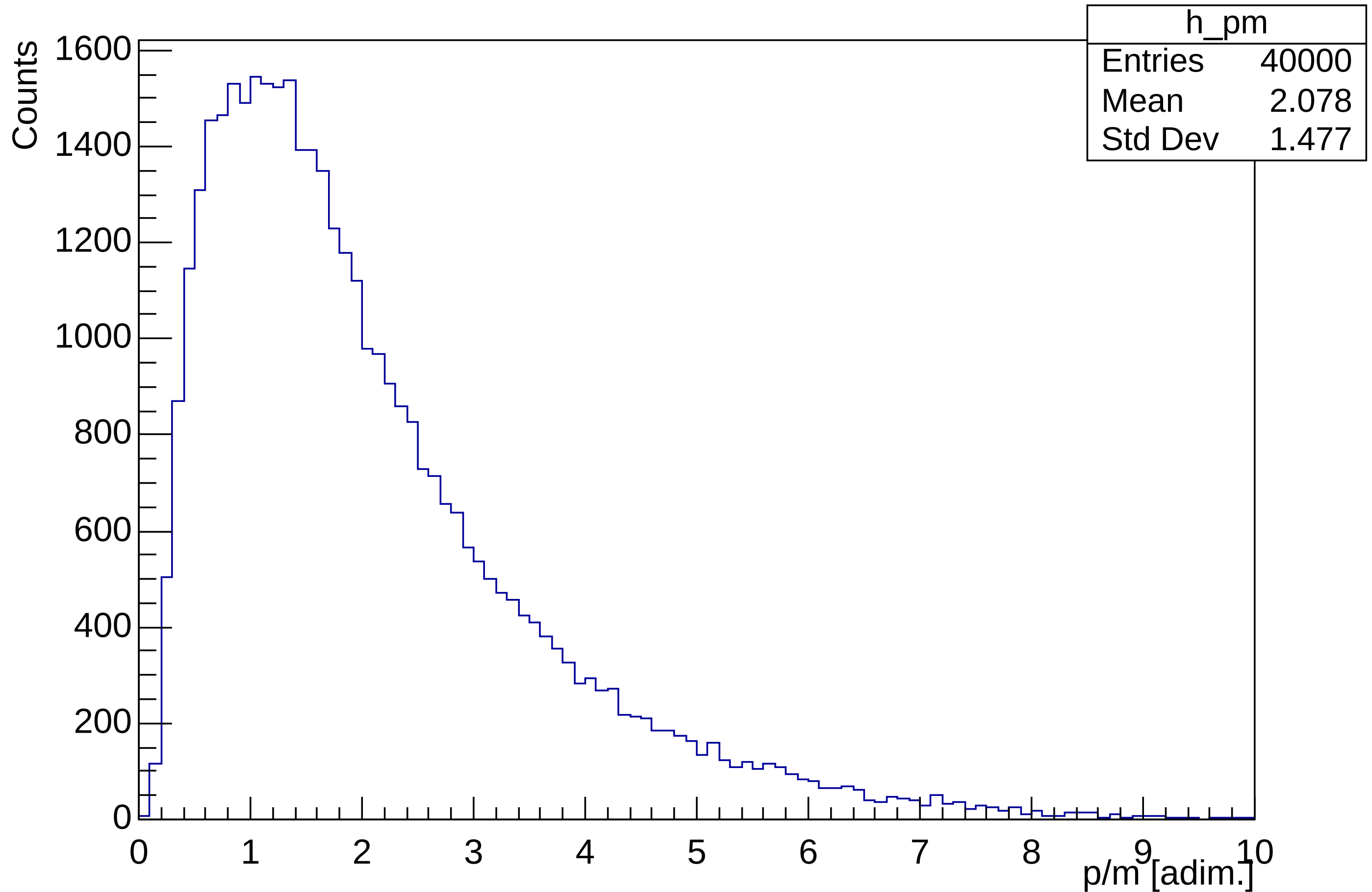
p/m (betagamma) distribution, gD=2, m=500 GeV
