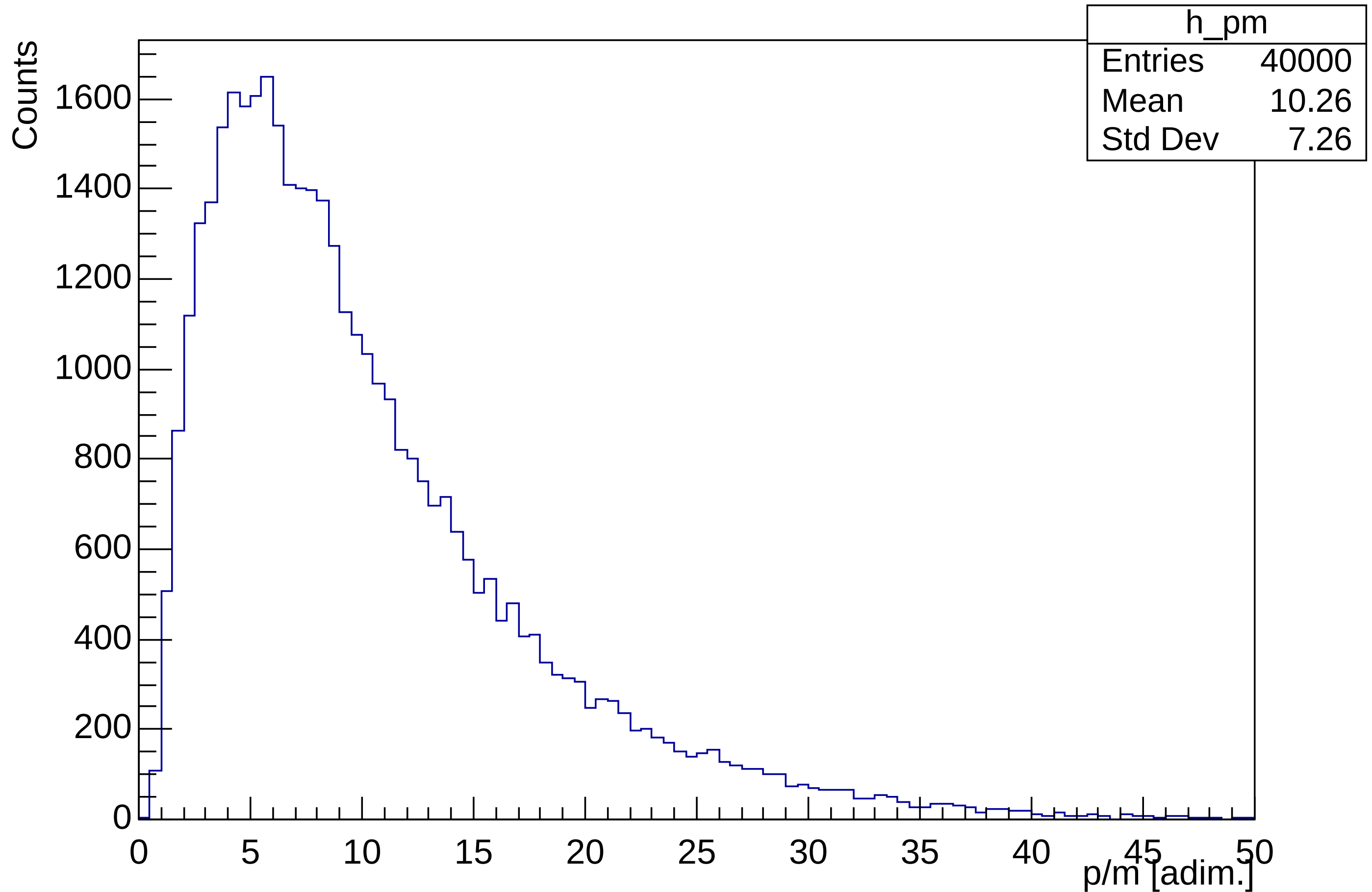
p/m (betagamma) distribution, gD=1, m=500 GeV
