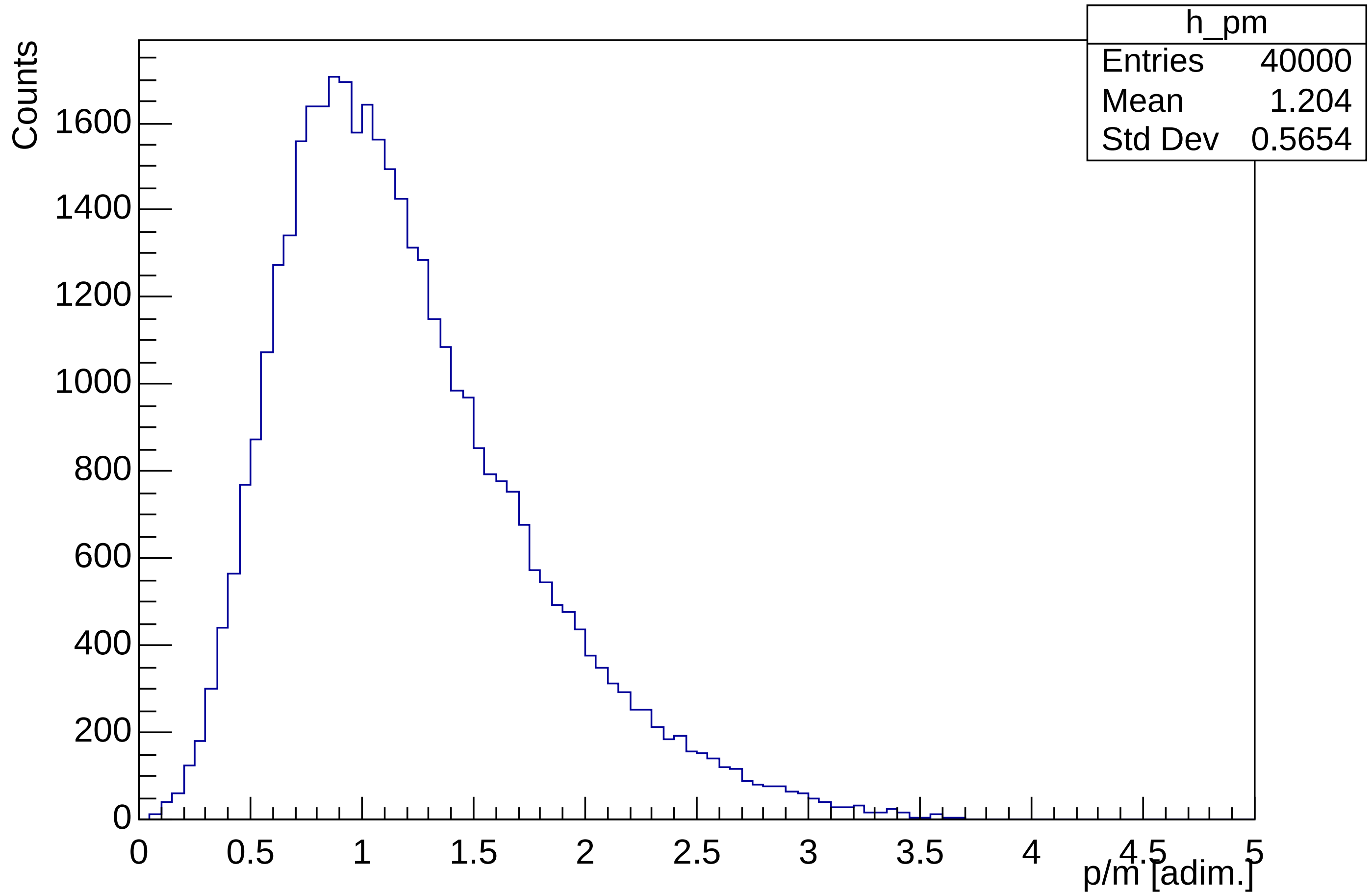
p/m (betagamma) distribution, gD=1, m=1500 GeV
