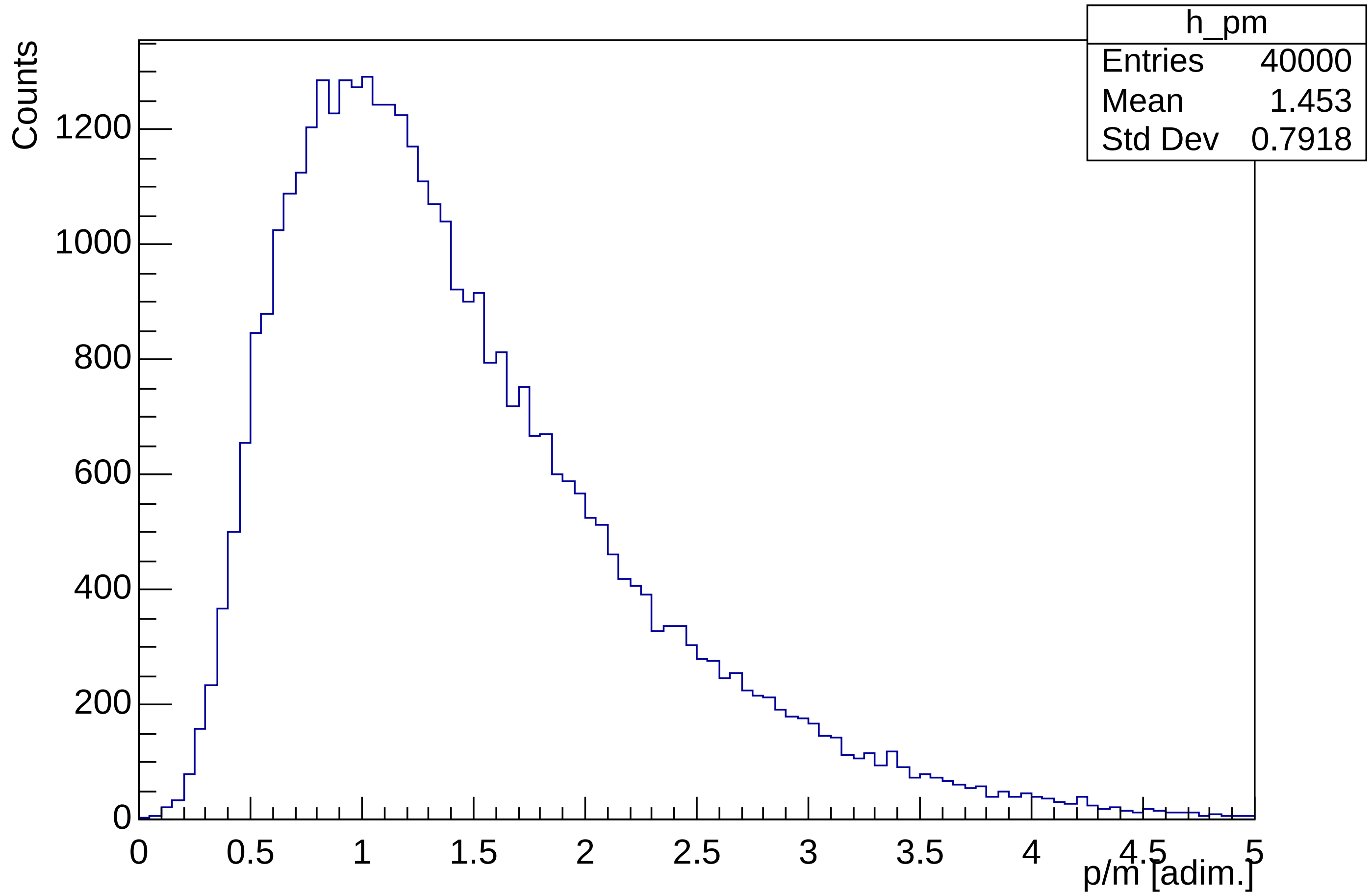
p/m (betagamma) distribution, gD=2, m=1000 GeV
