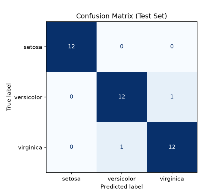
Confusion matrix
