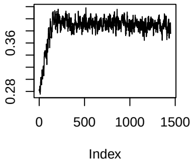
Trace plots 1–4 for admixture estimates ( k=5 )
