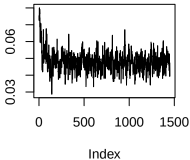
Trace plots 4–8 for admixture estimates ( k=5 )
