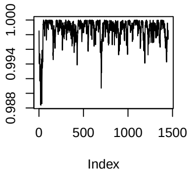
Trace plots 1–4 for admixture estimates ( k=6 )
