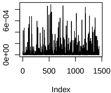
Trace plots 1–4 for admixture estimates ( k=6 )
