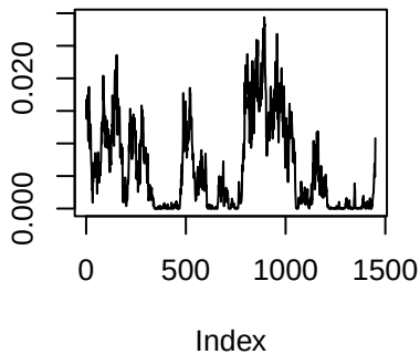
Trace plots 1–4 for admixture estimates ( k=7 )
