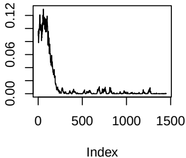
Trace plots 4–8 for admixture estimates ( k=7 )
