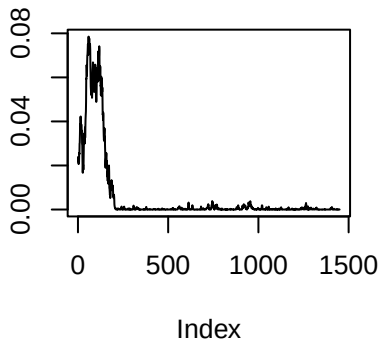
Trace plots 4–8 for admixture estimates ( k=7 )
