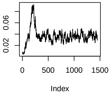
Trace plots 9–12 for admixture estimates ( k=7 )
