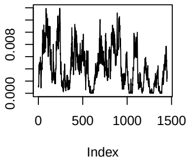
Trace plots 4–8 for admixture estimates ( k=9 )
