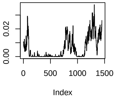
Trace plots for admixture estimates ( k=9 )
