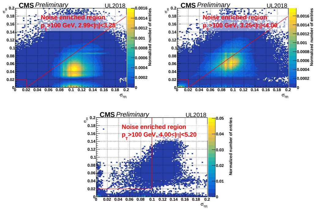
Figure 3.22: Two dimensional distribution of \sigma_{i\eta i\eta} and \sigma_{i\phi i\phi} in the noise-enriched region, split by the |\eta| of the jet. The first plot shows 2.99 < |\eta| < 3.25 interval, the second one shows 3.25 < |\eta| < 4 , and the last one shows 4 < |\eta| < 5.2 . The red lines on the plots indicate the cuts applied on these variables.
