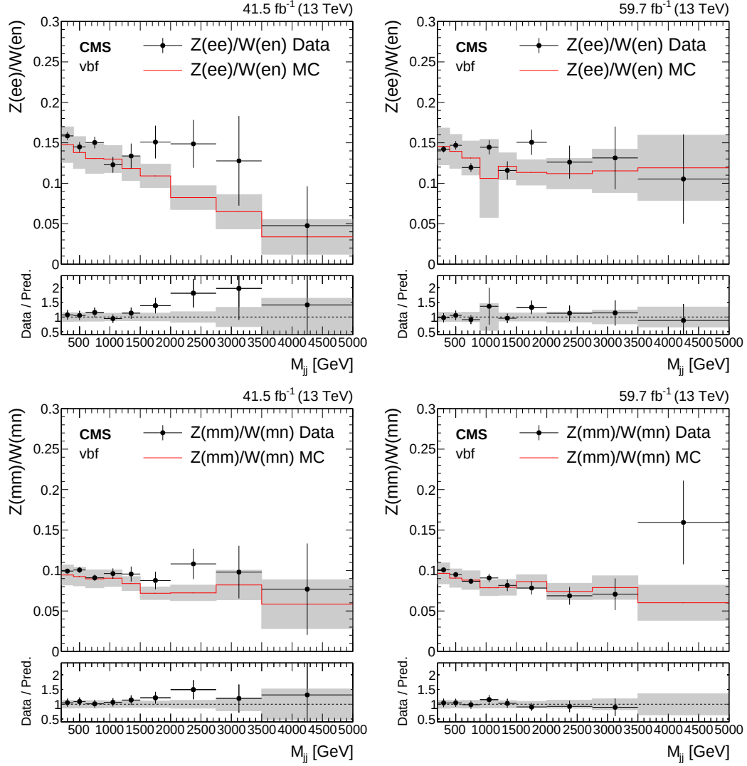
Figure 3-54: Transfer factors between Z and W control regions as a function of the dijet mass. Results for both 2017 (left) and 2018 (right) datasets are shown. Plots on the top row show the ratios between the electron regions, while the plots on the bottom show the ratios between muon regions. The bands show the theoretical and experimental systematic uncertainties on the ratios.
