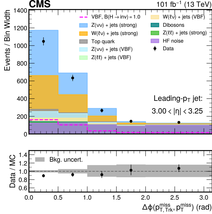
Figure 3.27: \Delta\phi(p_{T, \text{Trk}}^{\text{miss}}, p_T^{\text{miss}}) distribution for the closure test on the HF noise estimate. Events plotted here pass the VBF signal region selection, and have the leading jet in 3 < |\eta| < 3.25 range, where the HF noise contribution is highest. It can be observed, especially at high \Delta\phi(p_{T, \text{Trk}}^{\text{miss}}, p_T^{\text{miss}}) , the agreement between data and background yields is good after the residual HF noise estimation is taken into account. To account for residual differences, a 20% flat uncertainty is assigned to the HF noise template.
