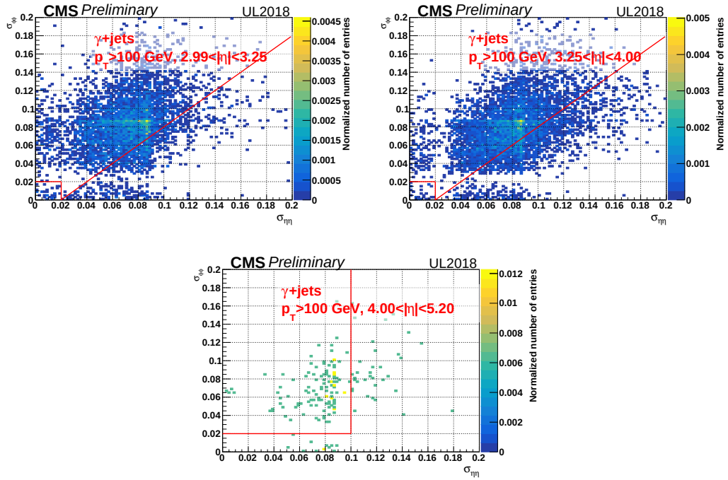
Figure 3.23: Two dimensional distribution of \sigma_{i\eta} and \sigma_{i\phi\phi} in the physics-enriched region, split by the |\eta| of the jet. The first plot shows 2.99 < |\eta| < 3.25 interval, the second one shows 3.25 < |\eta| < 4 , and the last one shows 4 < |\eta| < 5.2 . The red lines on the plots indicate the cuts applied on these variables.
