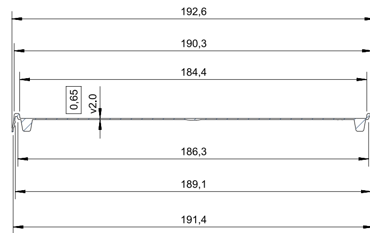
LENGTH SECTION S-S
