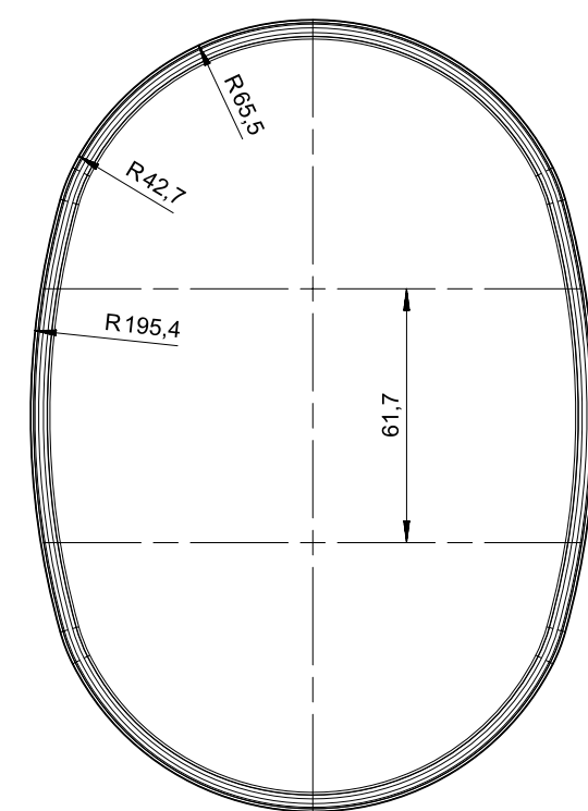
OUTSIDE VIEW
