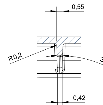
SECTION AD-AD
