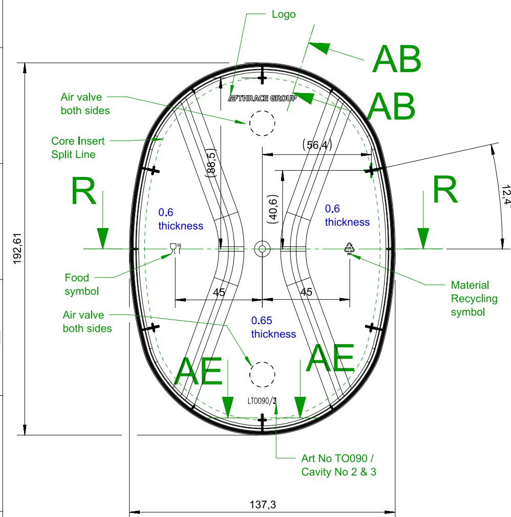
INSIDE VIEW
