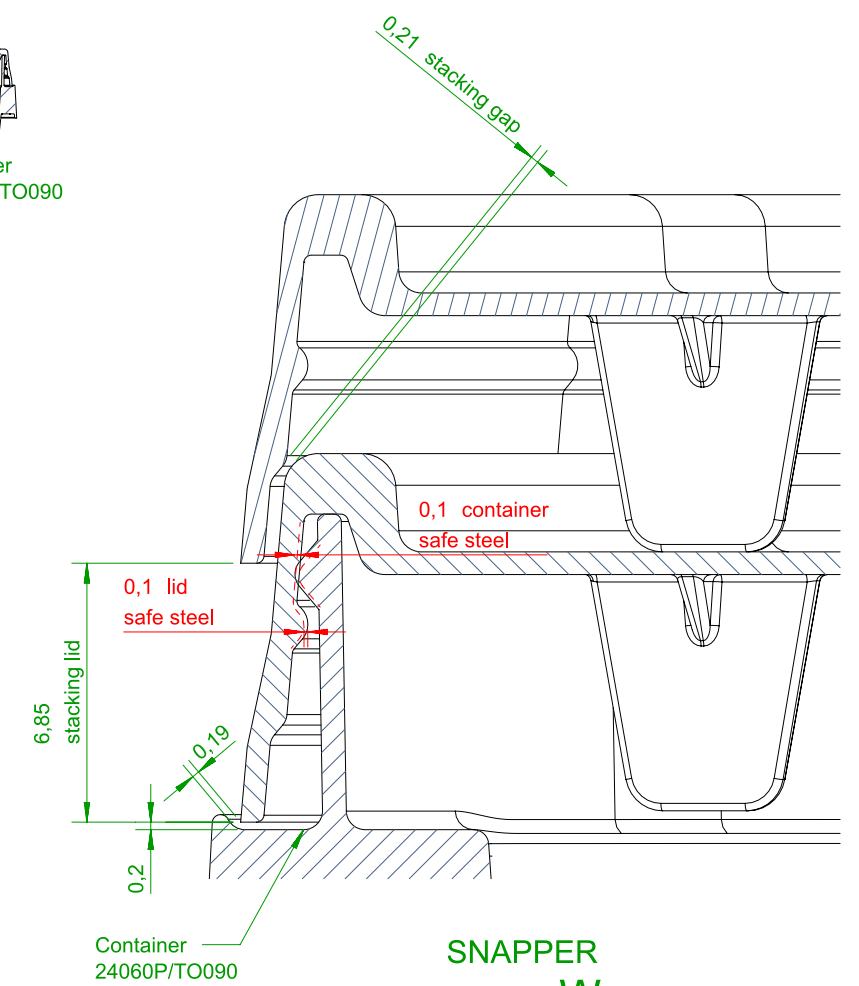
STACKING VIEW WITH CONTAINER LENGTH
