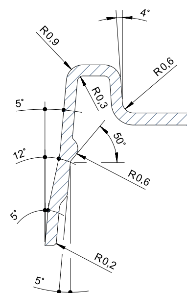
DETAIL AC
