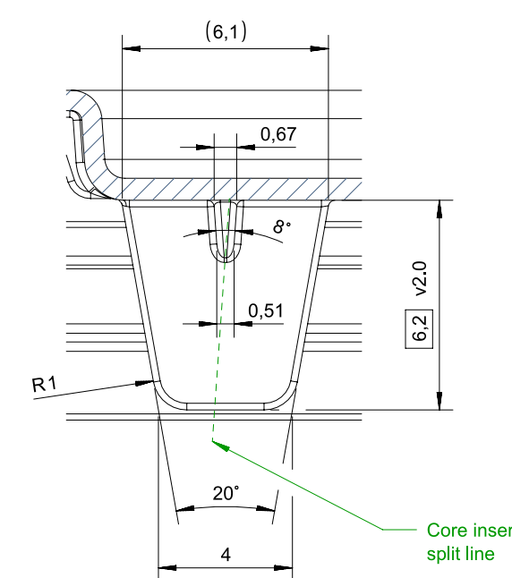
STACKING RIBS SECTION AF-AF
