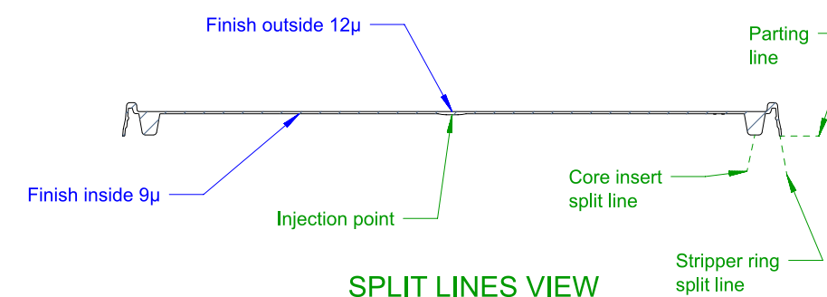
SPLIT LINES VIEW
